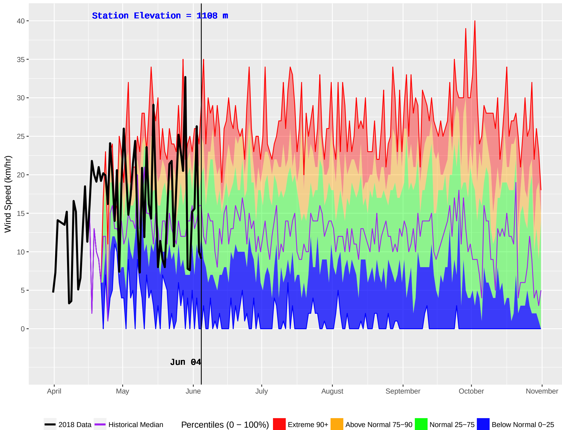
NABESHE (151) : Historical (1987–2016) and Current (2018) Noon Wind Speed
