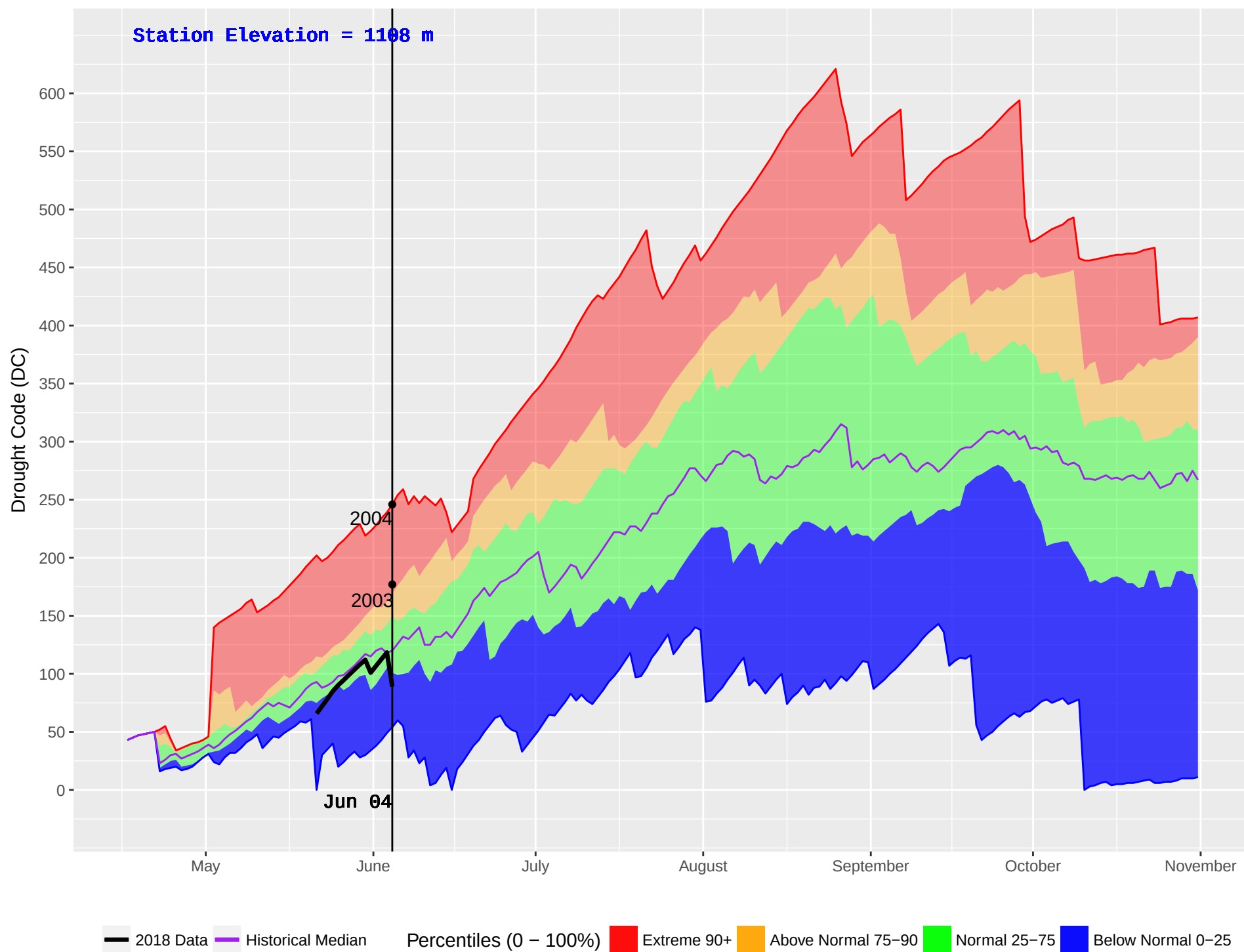
NABESHE (151) : Historical (1987–2016) and Current (2018) Noon Drought Code (DC)
