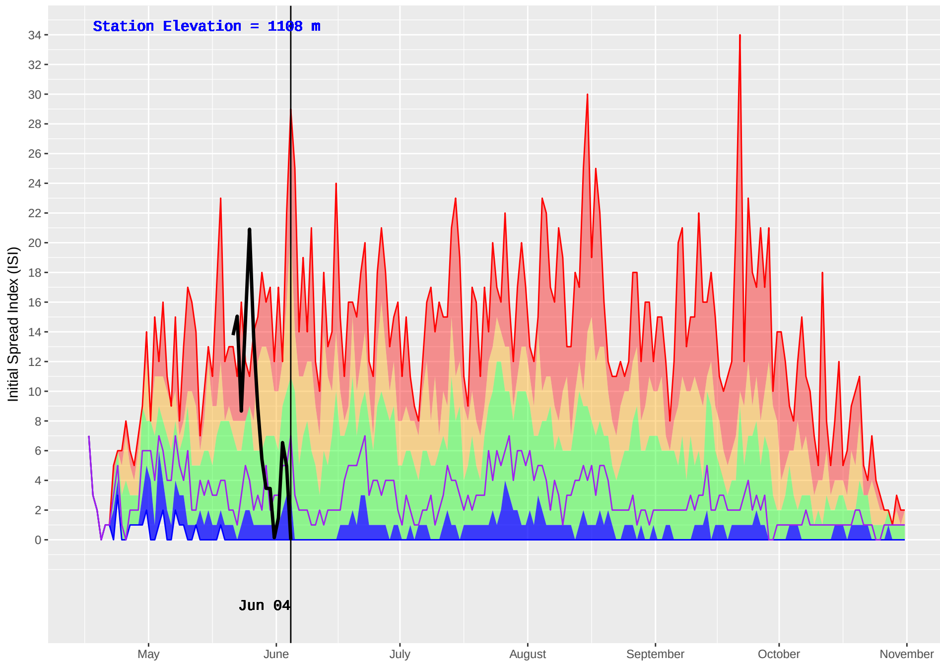
NABESHE (151) : Historical (1987–2016) and Current (2018) Noon Initial Spread Index (ISI)
