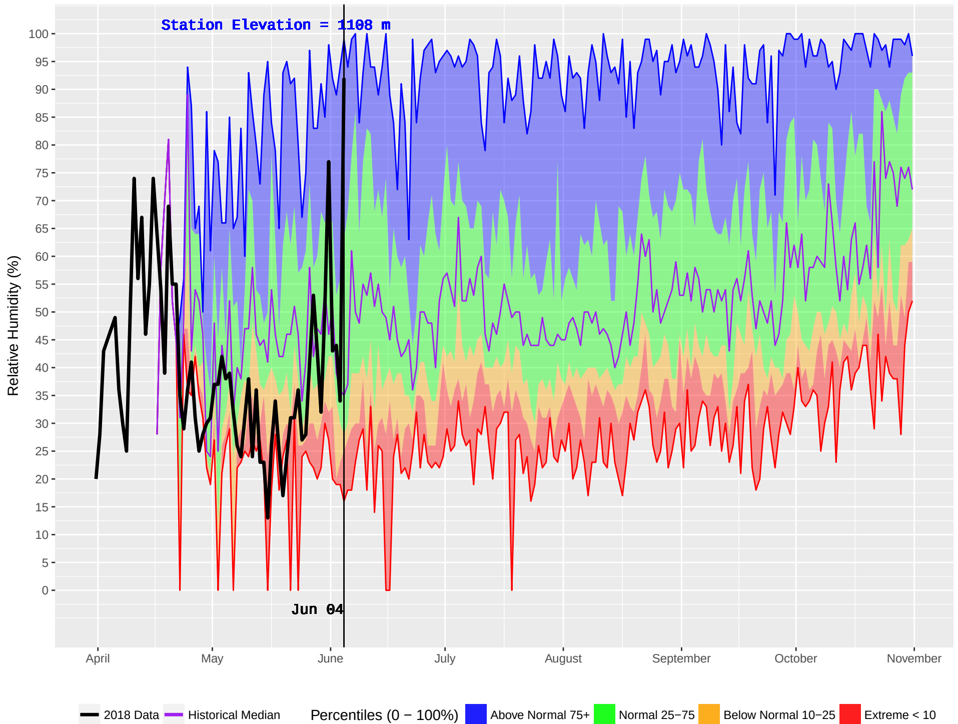
NABESHE (151) : Historical (1987–2016) and Current (2018) Noon Relative Humidity
