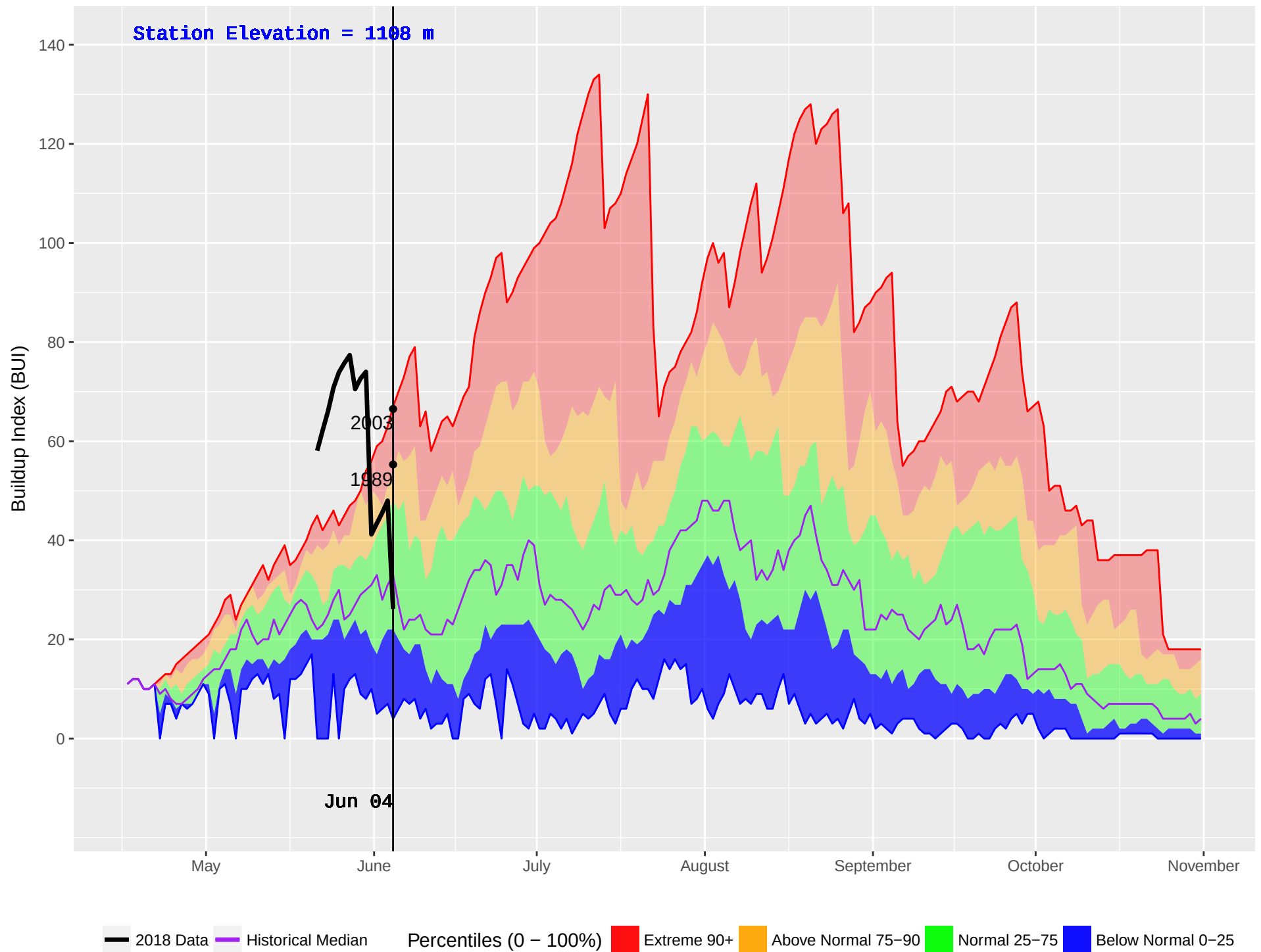
NABESHE (151) : Historical (1987–2016) and Current (2018) Noon Buildup Index (BUI)
