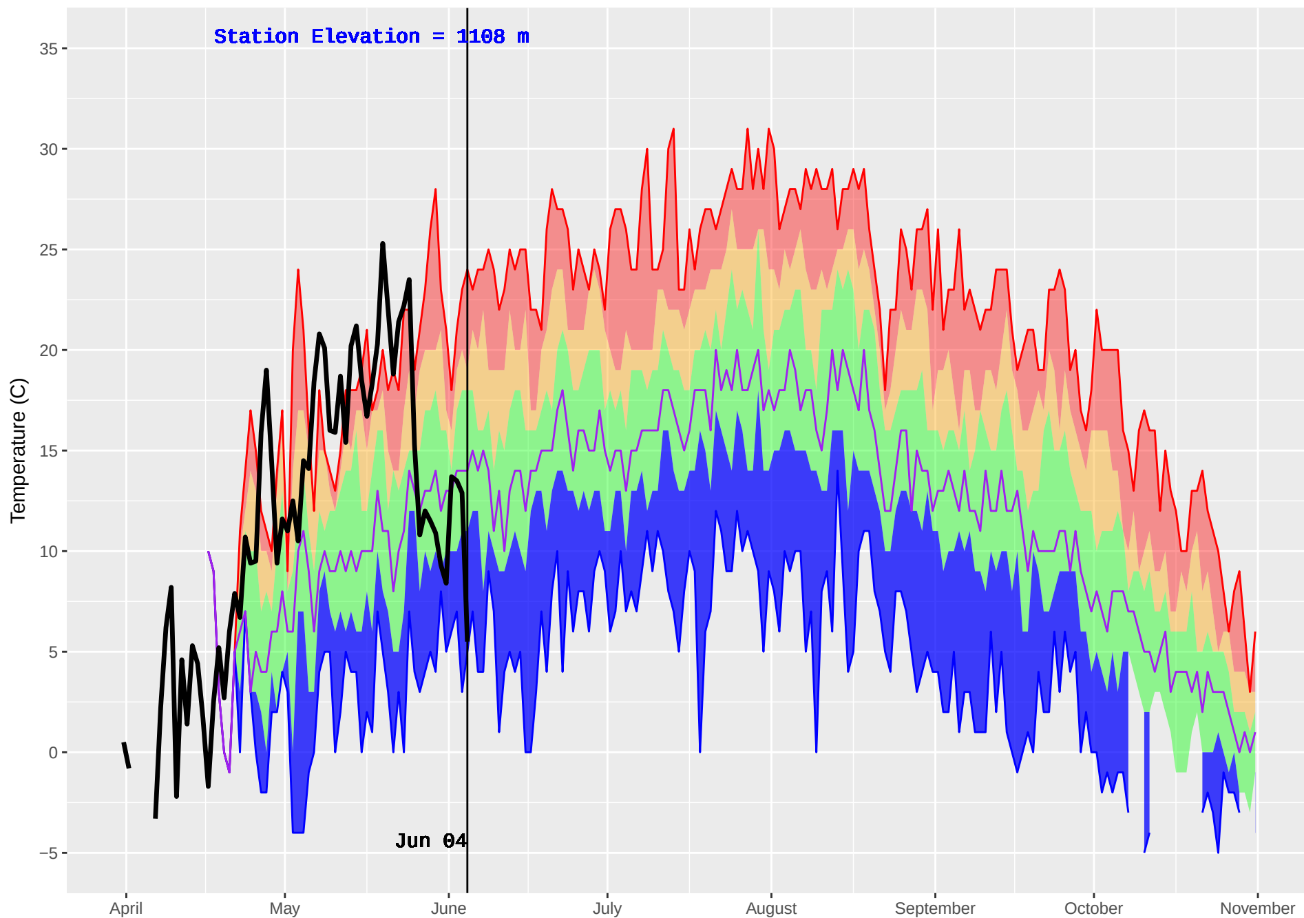
NABESHE (151) : Historical (1987–2016) and Current (2018) Noon Temperature
