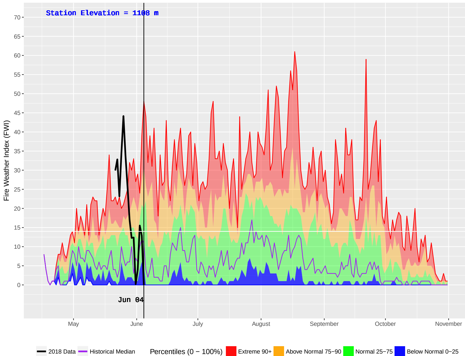
NABESHE (151) : Historical (1987–2016) and Current (2018) Noon Fire Weather Index (FWI)
